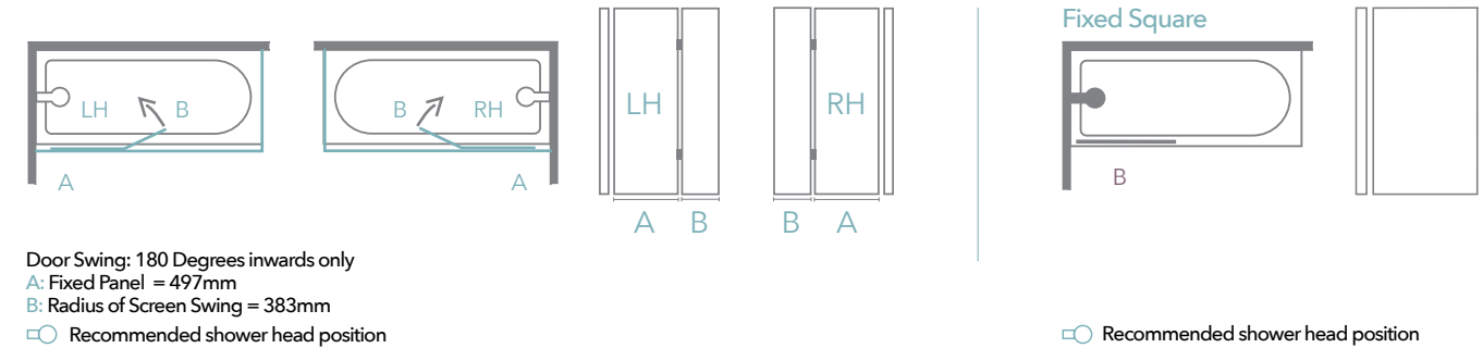
2 Panel Hinged Bath Screen
